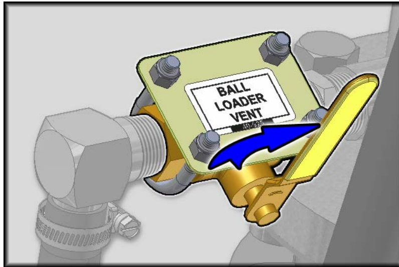
Figure 9 – Ball Loader Vent – Close Ball Valve
