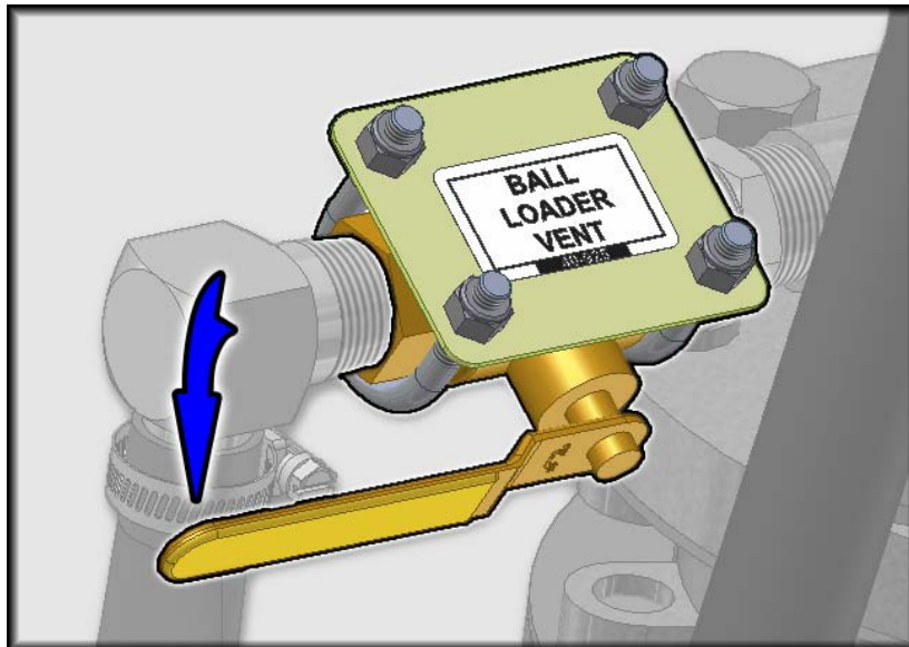
Figure 8 – Ball Loader Vent – Open Ball Valve
