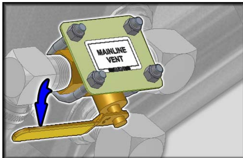
Figure 13 – Mainline Vent – Open Ball Valve
