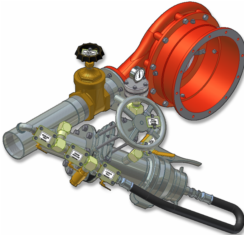
Figure 1 – Typical 4 Inch Clean-out Ball Launcher (PTO Version shown)
