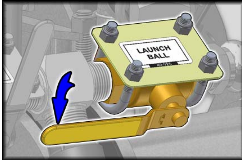
Figure 11 – Launch Ball – Open Ball Valve
