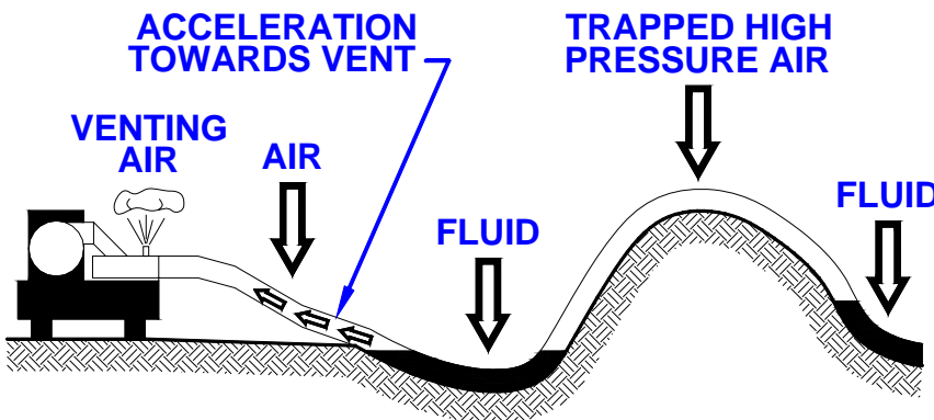
Figure 2 – Air-Fluid-Air Danger
