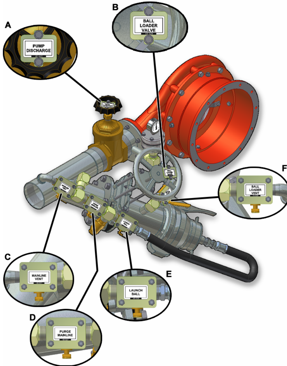
Figure 5 – 4 Inch Clean-out Ball Launcher Valve Layout
