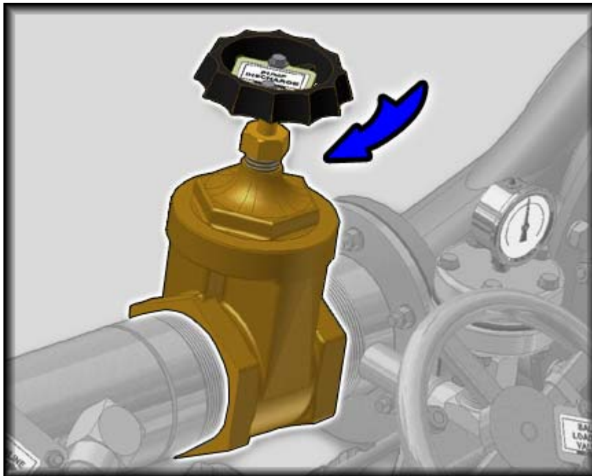
Figure 6 – Pump Discharge Valve – Close Gate Valve
